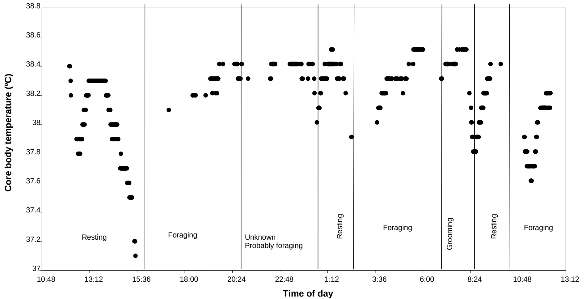
Figure 64. Representative profile of core body temperature of an adult male sea otter in relation to behavior and time of day. Each point represents the average core body temperature every 60 seconds. Corresponding behaviors are listed under the body temperature. Notice the pattern in temperature change over time for the same behaviors and change in behavior at temperature troughs
