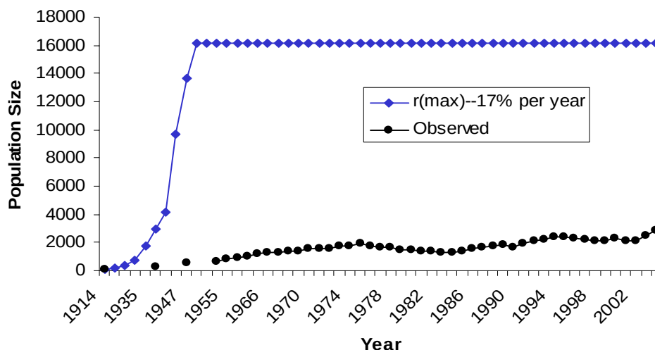
Figure 71. Trends in overall abundance of the southern sea otter population (circles) and a crude estimate of what this trend would have looked like if the population had increased at a rate of 17% \text{yr}^{-1} to an overall carrying capacity of 16,000 animals for the state waters of California (diamonds).
