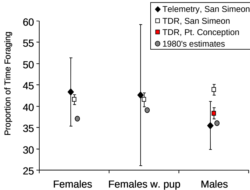
Figure 63. Temporal comparison of estimated proportion of time spent foraging by three groups of study animals, adult females without pups, adult females with pups, and adult males. Error bars indicate 95% confidence limits around the group means.
